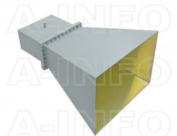
LB-1800-10-C-7/16F Standard Gain Horn Antenna 0.41-0.62GHz 10dB Gain 7/16(DIN) Female
